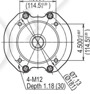
SAE CC 4 hole 4.500 +0.007 (114.5 +0.20 )
