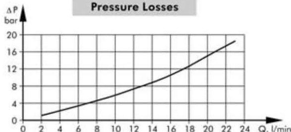
Pressure Losses
