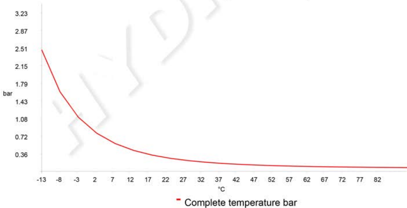
Delta P/T (Flow rate: 30 l/min)
