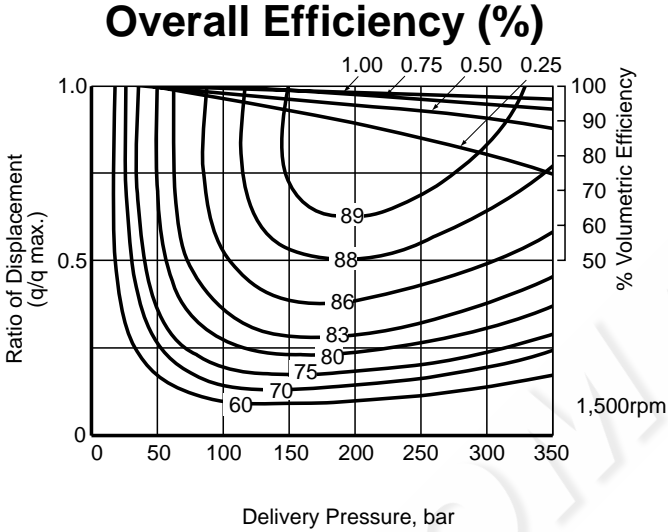
Performance Curves - K3VG280 and K3VG280 DT
