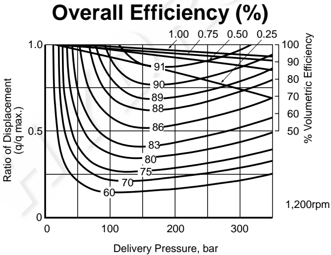
Performance Curves - K3VG280 and K3VG280 DT
