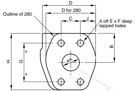
DELIVERY PORT
