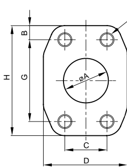
SUCTION PORT
