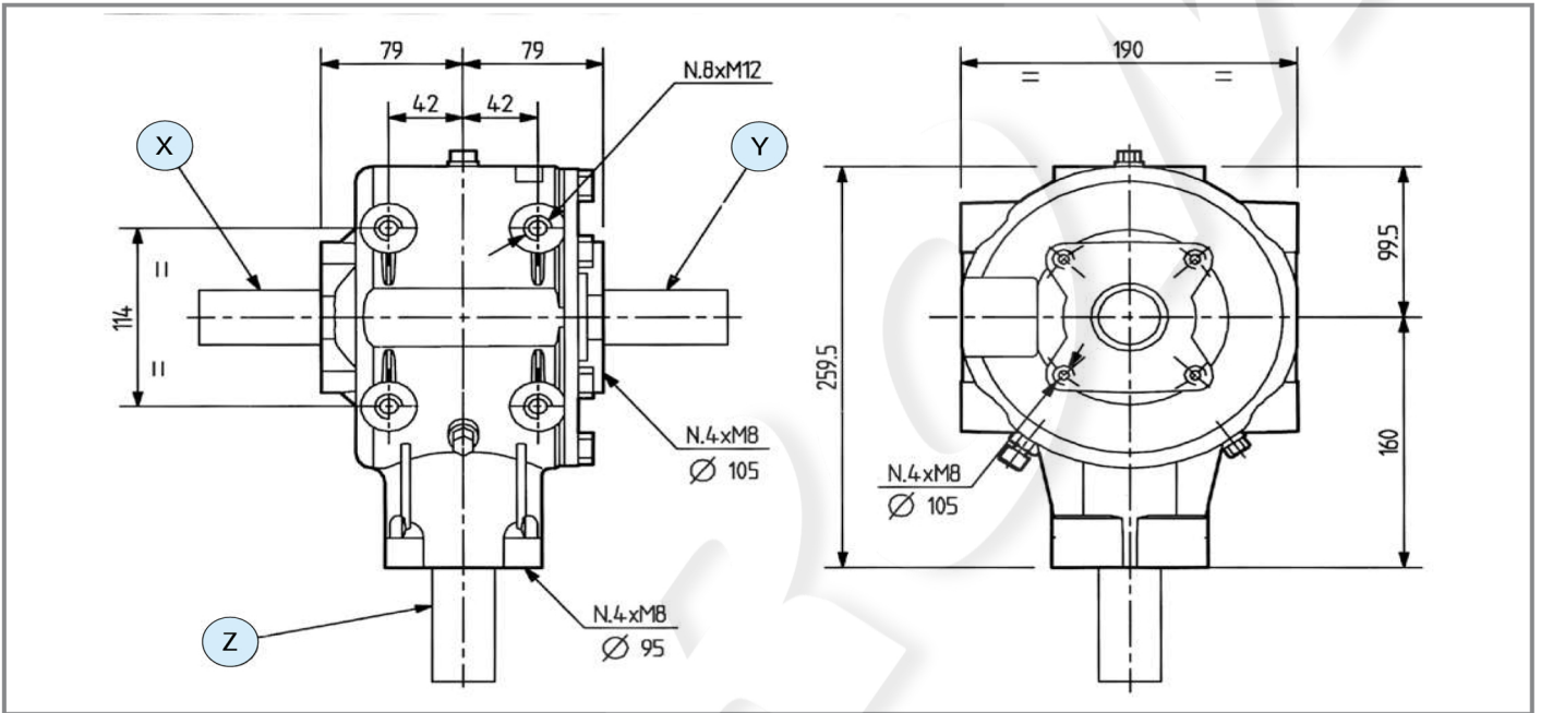
3 - Dentatura elicoidale / Helical Teeth
