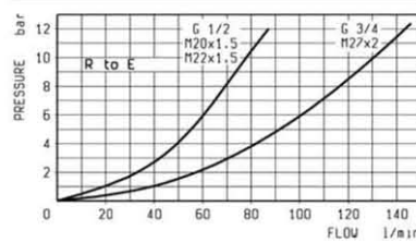
PRESSURE DROP
